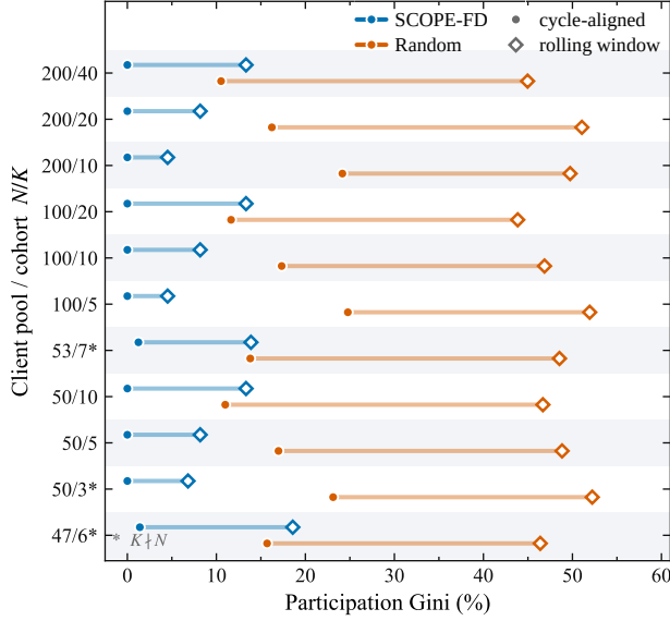
Fig. 6. Participation fairness across client-pool and cohort sizes on FMNIST over five seeds, one bar per selector. Filled circles are the cycle-aligned Gini coefficient at R = 100 ; open diamonds the rolling-window coefficient over a window offset from the participation cycle, so bar length shows how much the reading depends on window placement. Stars mark K \nmid N . Every value matches (17).
